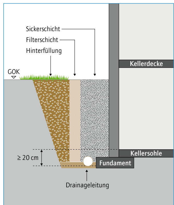
Abb. 52 – Drainage
